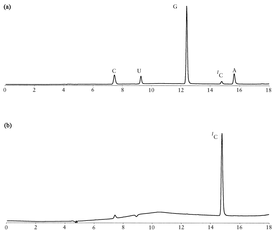
Figure 1. HPLC profile of: (a) enzymatic digestion mixture of r(5'-G I CUGGGCGCAGG-3'); and (b) 5-iodocytidine standard. The enzymatic digestion was performed with nuclease P 1 and calf intestine alkaline phosphatase. The HPLC column is Hypersil 5 \mu C18 (4.6 \times 250 mm). The mixture was eluted with triethylamine (100 mM, pH=7) and 50% methanol/100 mM triethylamine, with a linear gradient from 0 to 27.5% methanol (18 min) at a flow rate of 1 ml/min. The absorbance was detected at 254 nm. The extinction coefficients at 254 nm for C, U, G, I C and A were 7.0 \times 10 3 , 9.3 \times 10 3 , 13.5 \times 10 3 , 4.2 \times 10 3 , 13.4 \times 10 3 , respectively. The retention times of C, U, G, I C and A were 7.49, 9.33, 12.49, 14.89 and 15.76 mins, respectively. The ratio of peak areas measured after correction for extinction coefficients at 254 nm of C, U, G, I C and A are 2.18:1.00:6.70:0.77:1.06, respectively, with standard errors of \pm 10–20%
